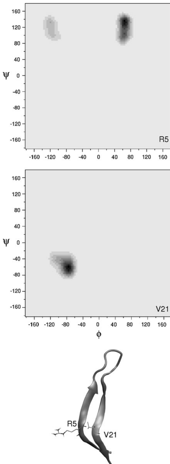
Fig. 5 Analysis of the kink in the backbone. Top panel Ramachandran plot of R5. Middle panel Ramachandran plot of V21. Bottom panel representative hairpin structure. The results refer to the simulation in water. Similar results are also observed along the 1.1 \mu s-long simulation in mixed solvent
