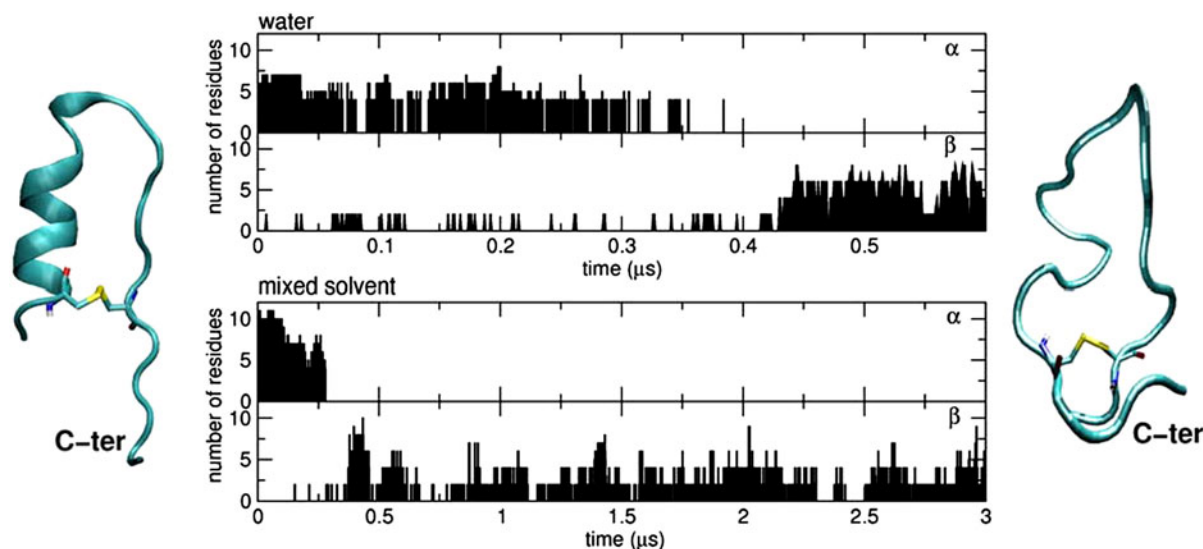
Fig. 2 Time-evolution of the secondary-structure content of LfcinB along the two simulations started from the \alpha -helical conformation in water ( top ) and in membrane-mimicking mixture ( bottom ). The secondary-structure content was
