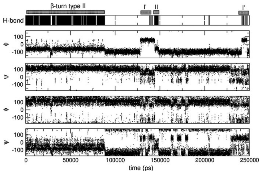
Fig. 4 Top panel existence of the turn hydrogen bond between residue i th (K12) and (i + 3) th (A15) along the simulation in water. Bottom panels \phi/\psi torsion angles of the (i + 1) th residue (L13) and (i + 2) th (G14) along the simulation in water. Similar results are also observed along the 1.1 \mu s-long simulation in mixed solvent
