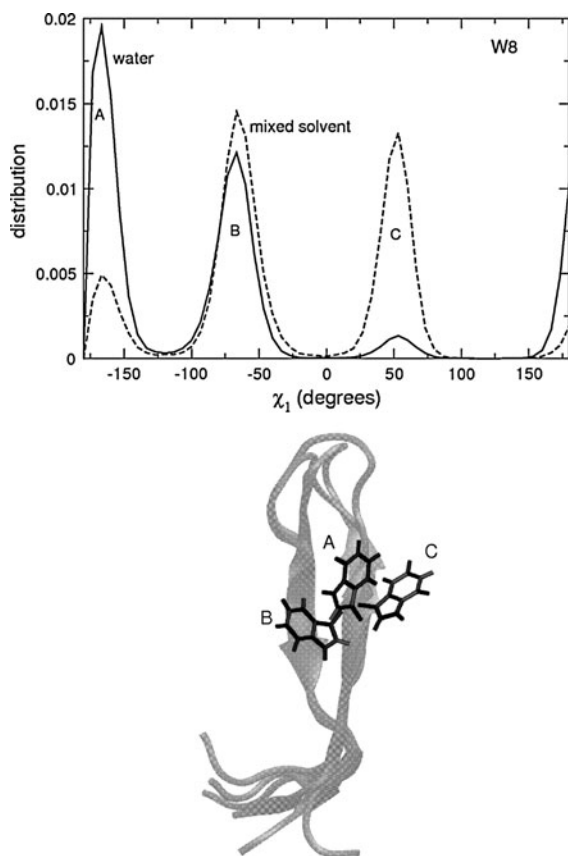
Fig. 7 Top panel distribution of the \chi_1 torsion angle of the side-chain of W8 in the simulations in water (solid line) and in mixed solvent (dashed line). Bottom panel representative conformations of the side-chain of the three main peaks A, B and C
