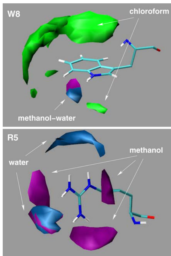
Fig. 9 Spatial distribution function (Kulińska et al. 2000) for chloroform, methanol and water around residue W8 ( top ) and residue R5 ( bottom ) calculated over the 1.1 \mu s-long MD trajectory of the \beta -hairpin in mixed solvent. Each curve represents an isosurface in the local coordinate system around the residue in which the local concentration of the corresponding solvent component is 50% of the maximum value of the distribution function. Hydrophilic residues, as R5, are mainly surrounded by methanol and water, while hydrophobic residues, as W8, show a preference for chloroform
