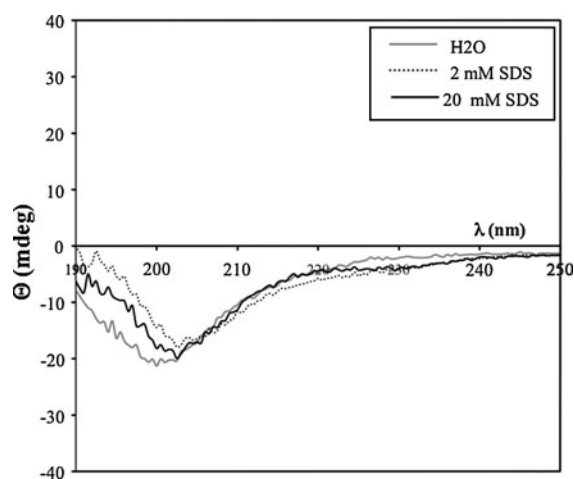
Fig. 1 The CD spectra of LfcinB (100 \mu M) in water, 2 mM non-micellar SDS and 20 mM micellar SDS solution at 25°C
