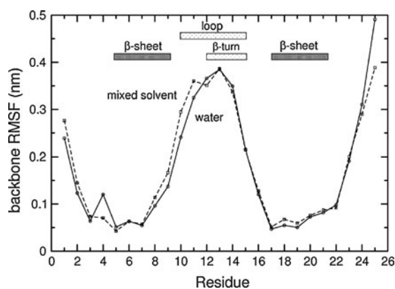
Fig. 3 Root mean square fluctuation (RMSF) of the backbone atoms in the simulations in water ( solid line ) and in mixed solvent ( dashed line )
