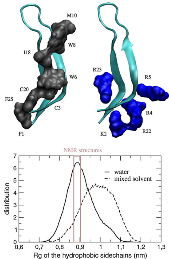
Fig. 6 Analysis of the side-chains. Top panel representative structure of the hydrophobic side-chains forming the hydrophobic surface, i.e., residues 1, 3, 6, 8, 10, 18, 20 and 25 ( left ) and of the hydrophilic side-chains that are on the opposite side of the hydrophobic surface, i.e., residues 2, 4, 5, 22 and 23 ( right ) along the simulation in water. Bottom panel radius of gyration ( R_g ) of the above mentioned hydrophobic side-chains in water ( solid line ) and in mixed solvent ( dashed line ). The interval highlighted in the box indicates the range of radius of gyration of the hydrophobic side-chains in the 20 NMR (Hwang et al. 1998) structures in water
