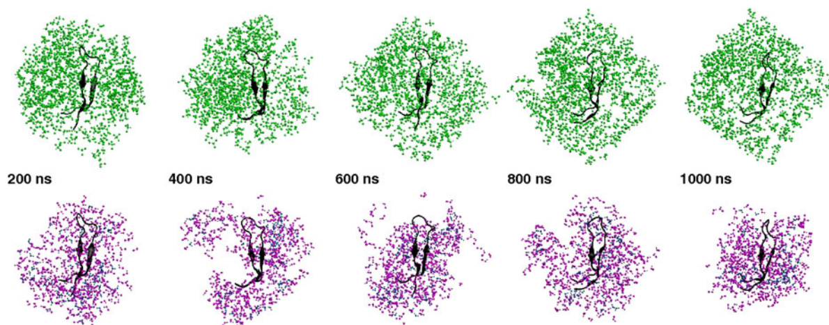
Fig. 8 Snapshots along the 1.1 \mu s-long MD trajectory of the \beta -hairpin in mixed solvent showing the variation of the clusters in the mixture. Chloroform and methanol/water molecules are shown in the top and bottom panels, respectively
